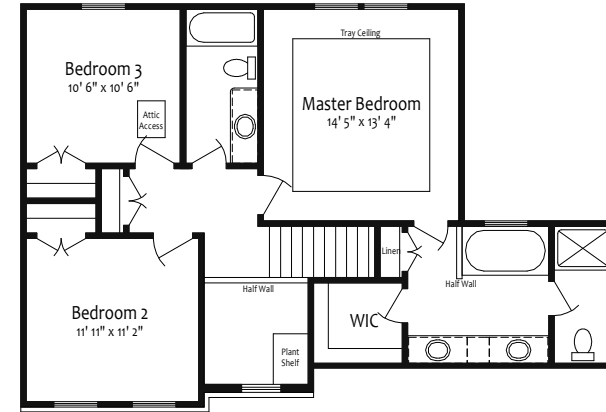
Second Floor 8' Ceilings 852 Sq Ft
